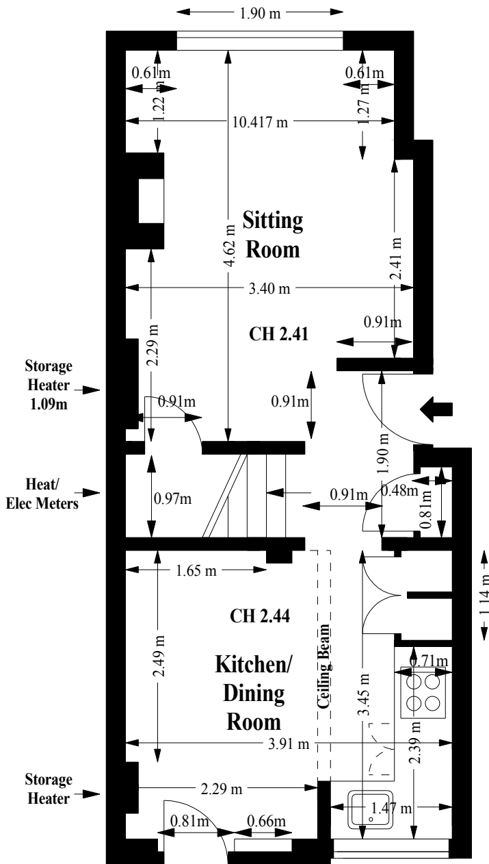
Ground Floor
